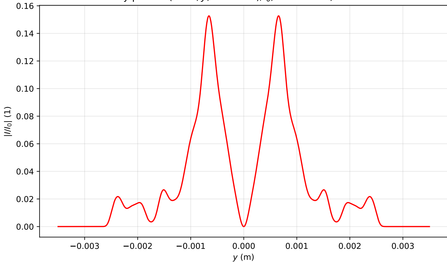
Intensity profile I(x=0, y, z=2.946)/I_0 , \text{Pin}=9.0\text{Pcr} , artificial time
